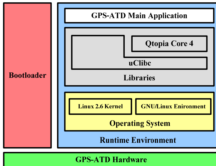
Figure 26: GPS-ATD firmware architecture
