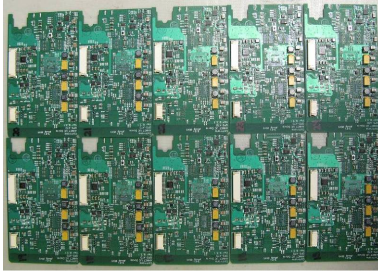
Figure 24: Fully-assembled GPS-ATD bottom-side circuit boards (qty 10 shown)
