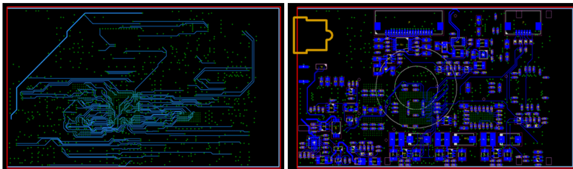
Figure 18: Layer 4 and layer 5 of the GPS-ATD circuit board
