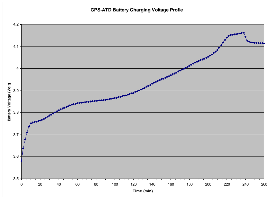
Figure 30: GPS-ATD battery charging curve
