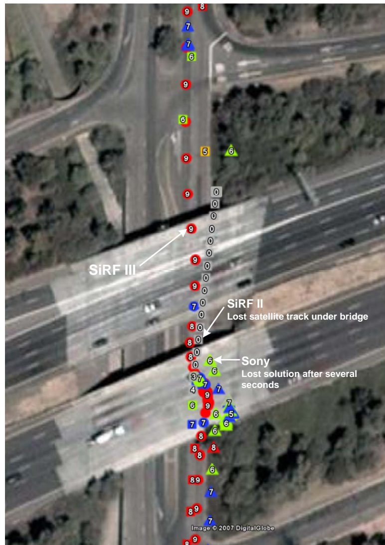
Figure 8 Bridge test results for SiRF II, SiRF III and Sony GPS receivers (number on symbol indicates number of satellites used for position calculation)
