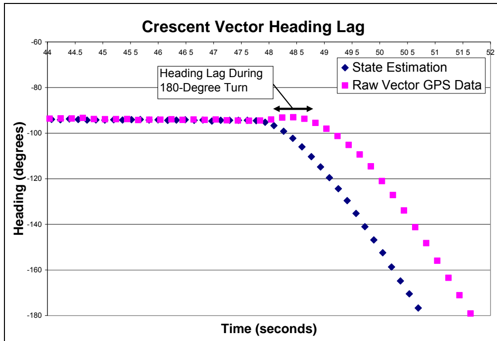
Figure 5.3 Crescent Vector GPS heading lag during a turn
