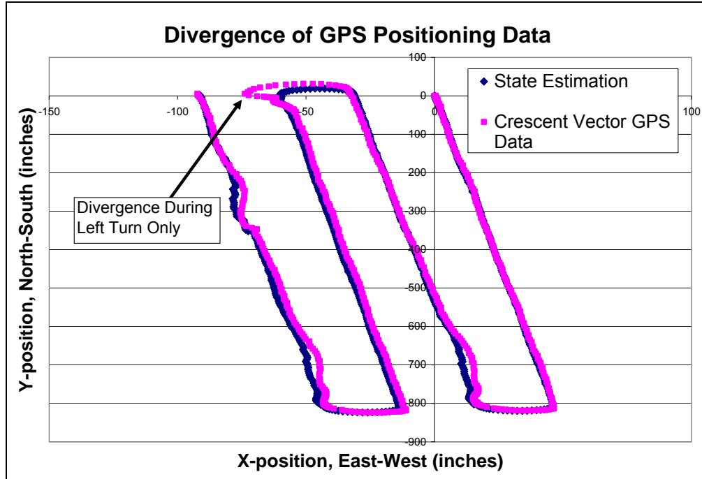
Figure 5.4 Crescent Vector GPS positioning divergence
