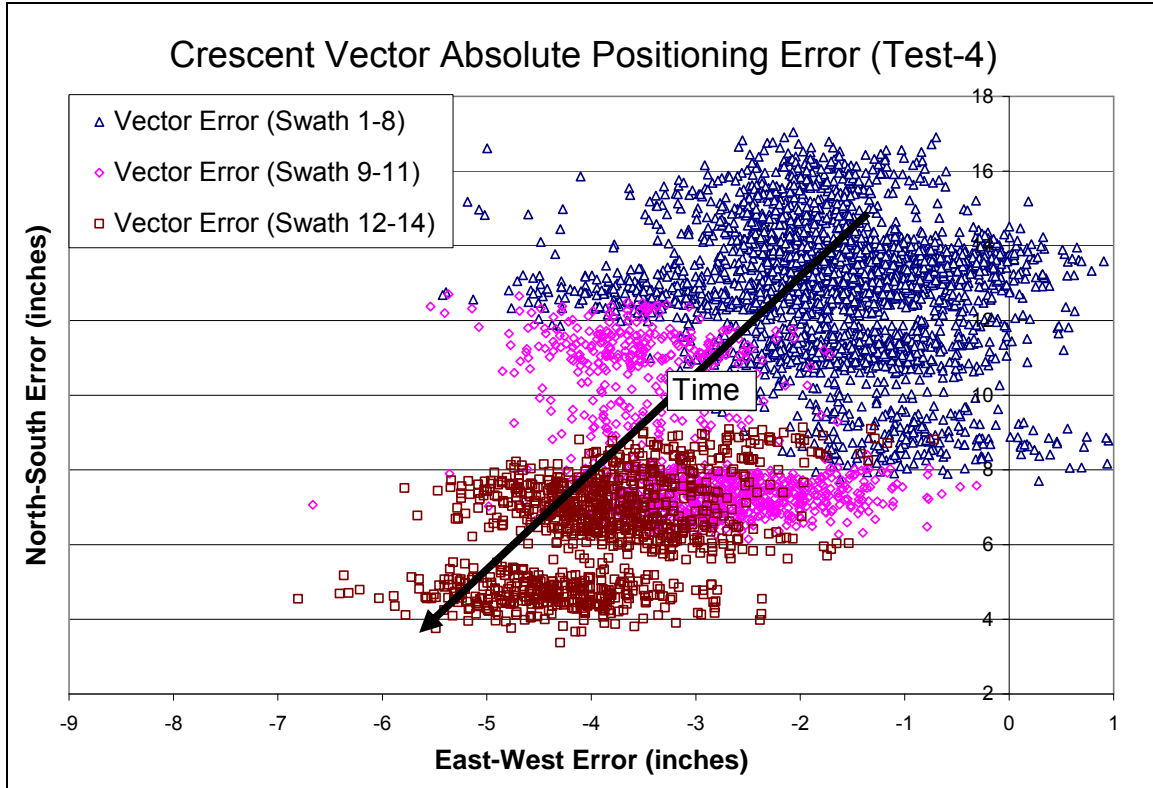
Figure 5.12 Crescent Vector absolute dynamic positioning error
