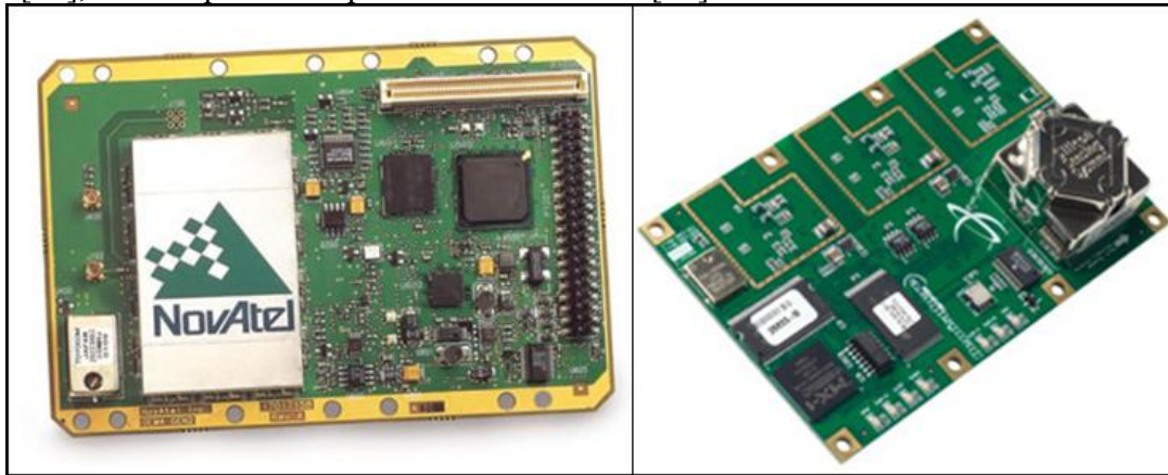
Figure 4.2 NovAtel OEMV-4 (left), Crescent Vector OEM (right)
