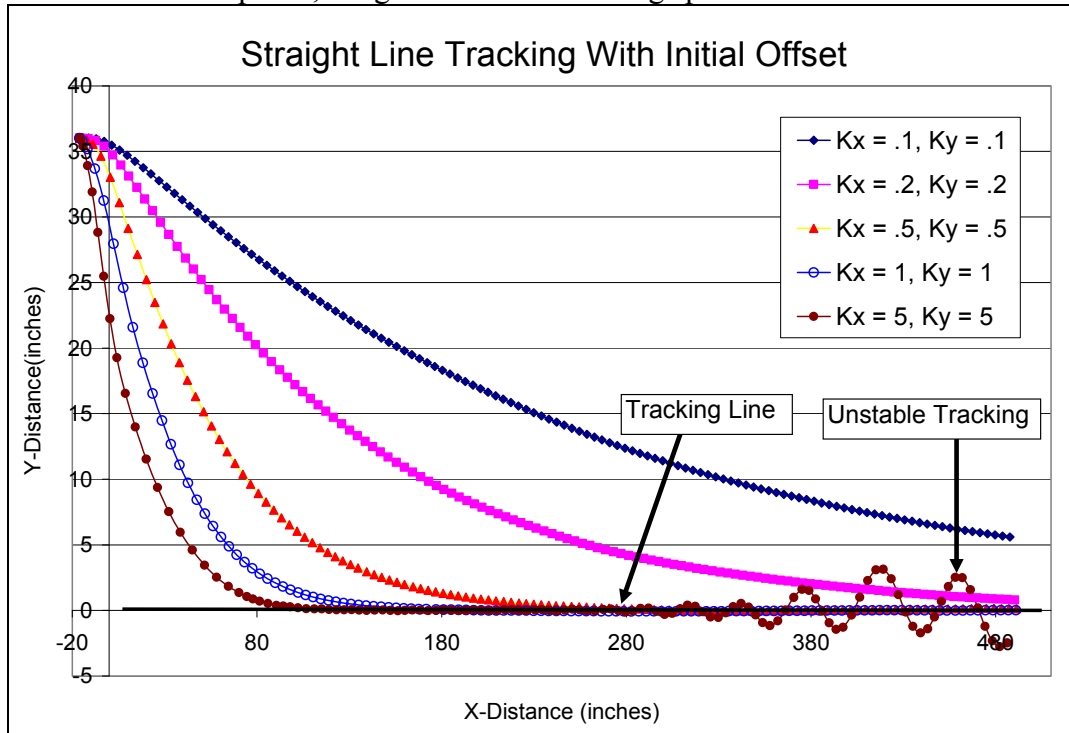
Figure 4.14 Tracking of a straight line trajectory with a horizontal offset of 36 in (91 cm)
