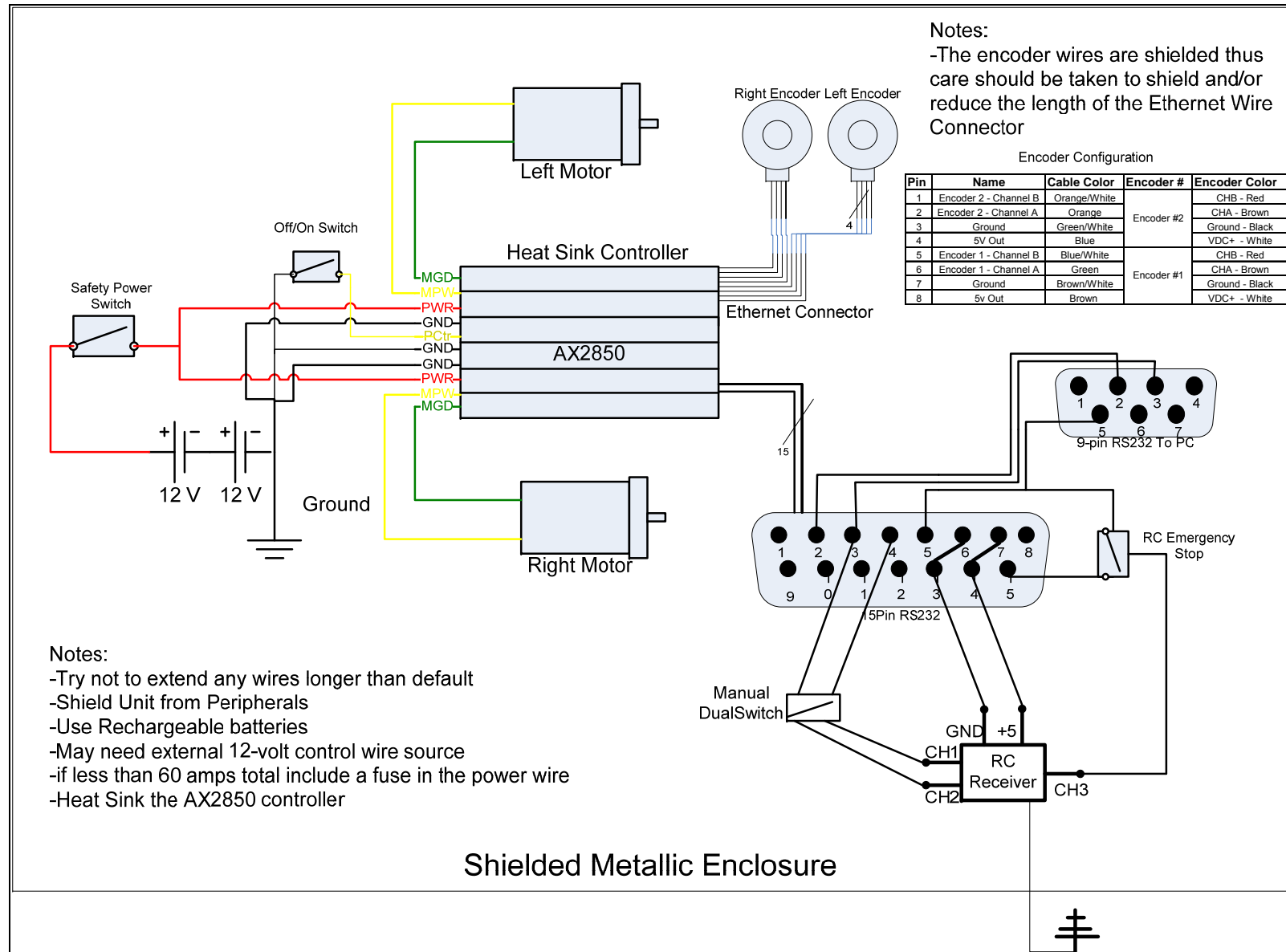
Figure A.6 Motor controller circuit design
