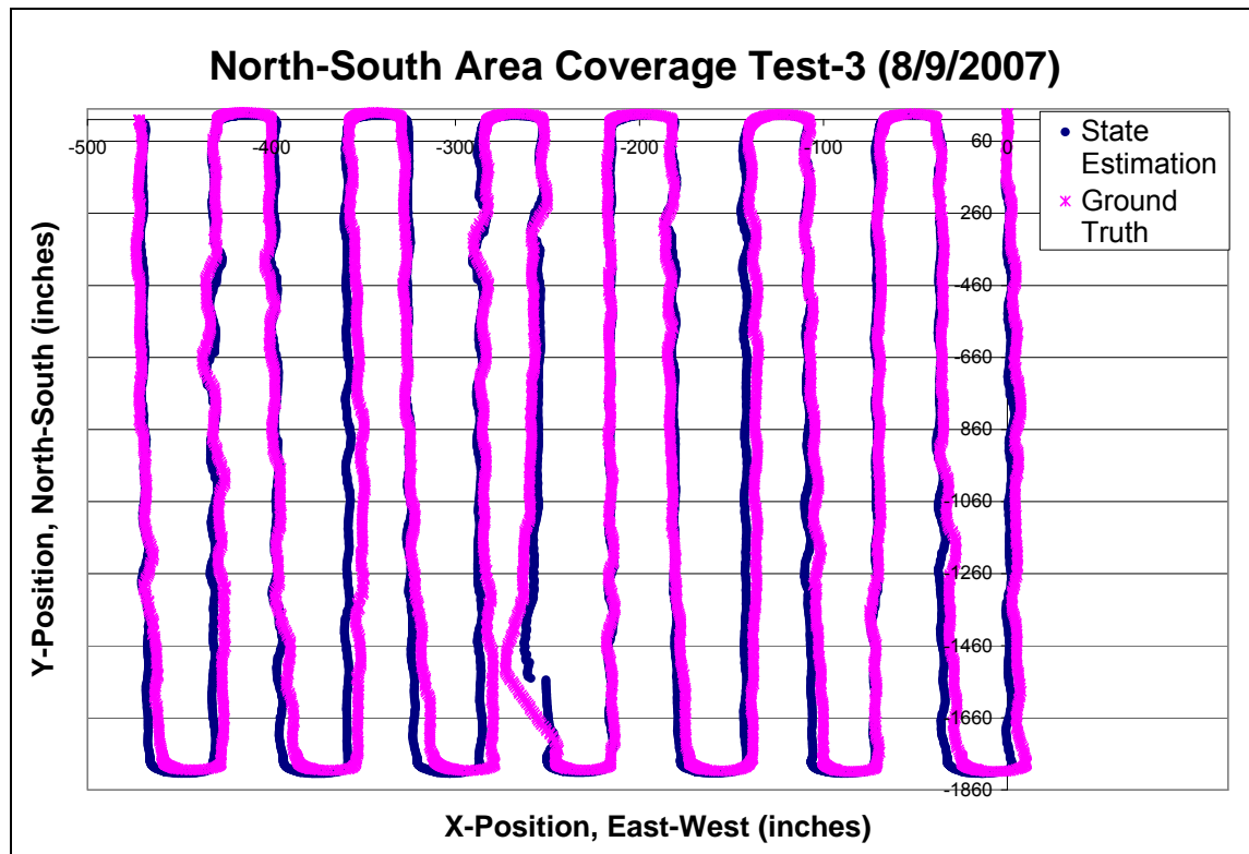
Figure C.3 Path tracking results from Test-3
