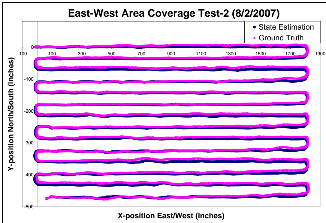
Figure C.2 Path tracking results from Test-2
