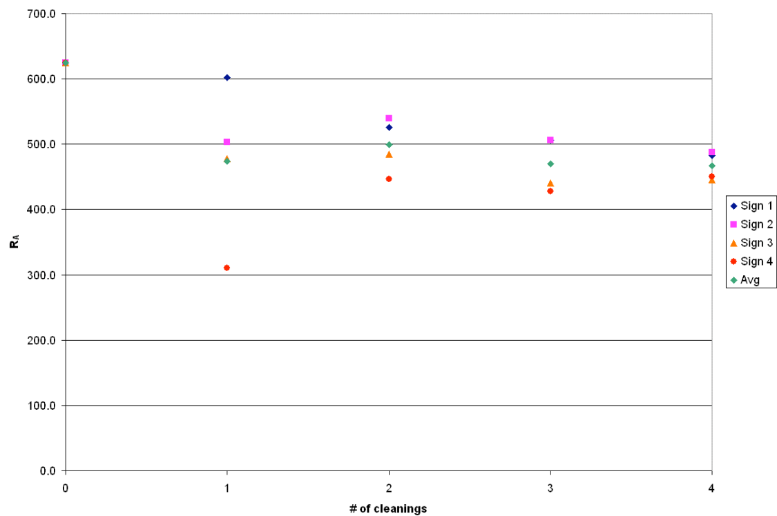
Figure 3-24: Multiple cleanings on painted signs with 1160
