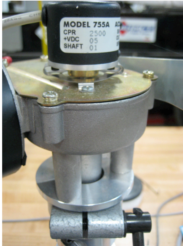
Figure 3-14: Encoder attached to back of motor
