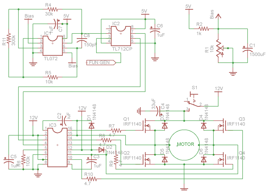
Figure 3-13: Class D PWM driver schematic
