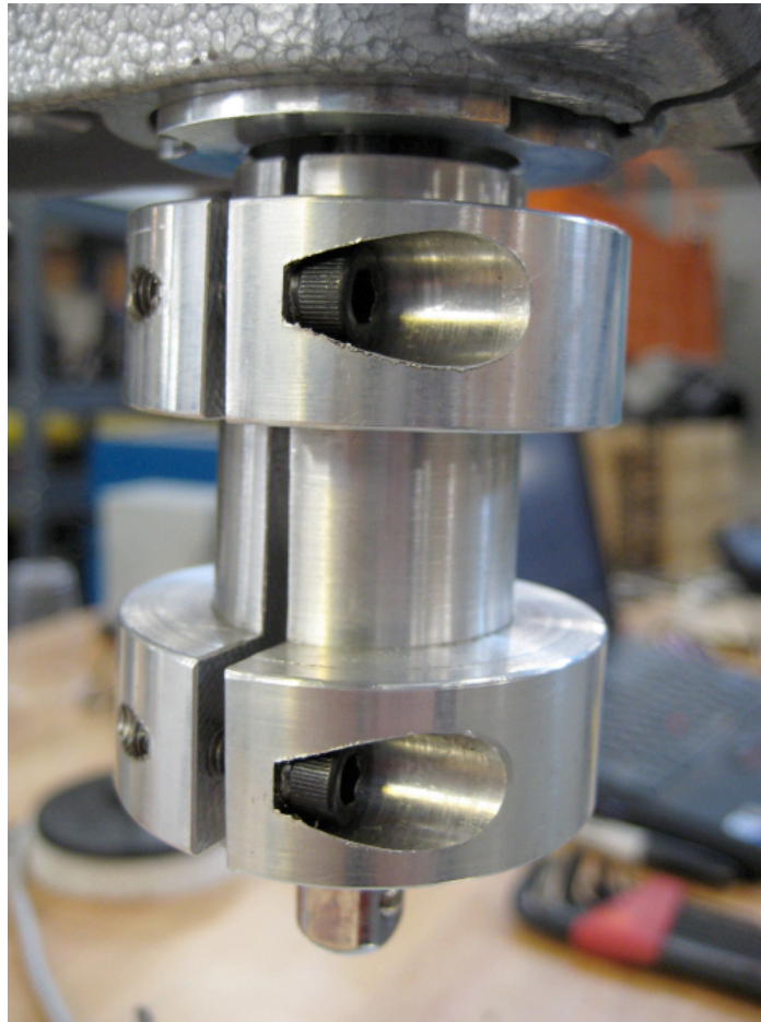
Figure 3-6: Coupling from shaft to brush
