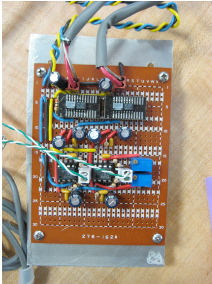
Figure 3-15: Filtration and amplification circuit for instrumentation
