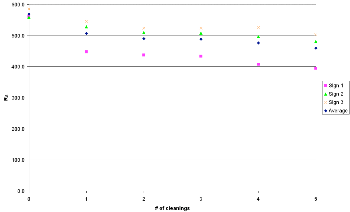
Figure 3-21: Results from multiple runs w/o 1160 film
