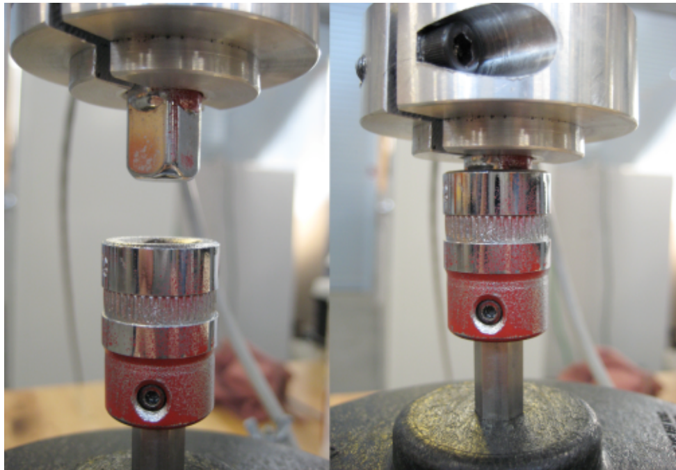
Figure 3-7: Brush connection to clamp-on coupler
