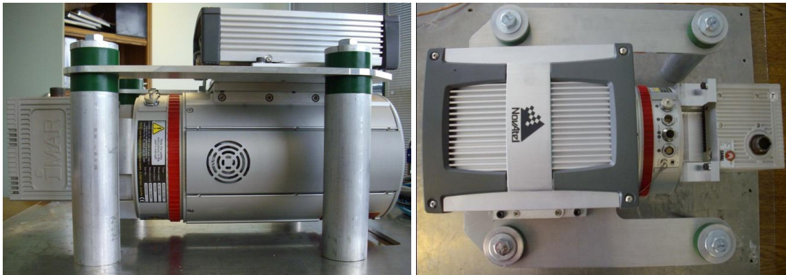
Figure A.6: Eagle Mapping aerial LiDAR system
