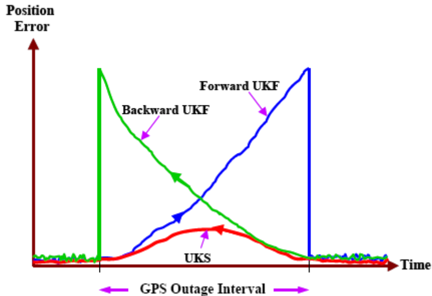
Figure A.4: Positional error comparison of Forward KF, Backward KF, and Combined Forward and Backward KF (UKS) solutions [20]
