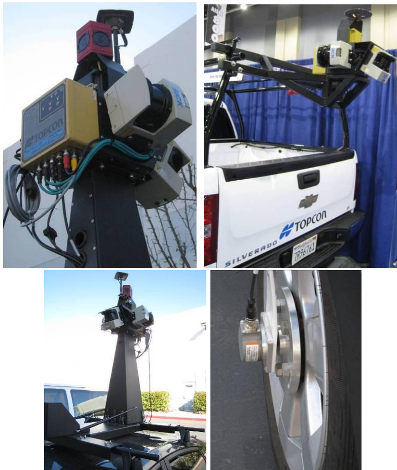
Figure A.23 Topcon IPS-2 system configured with SICK LiDAR scanners
