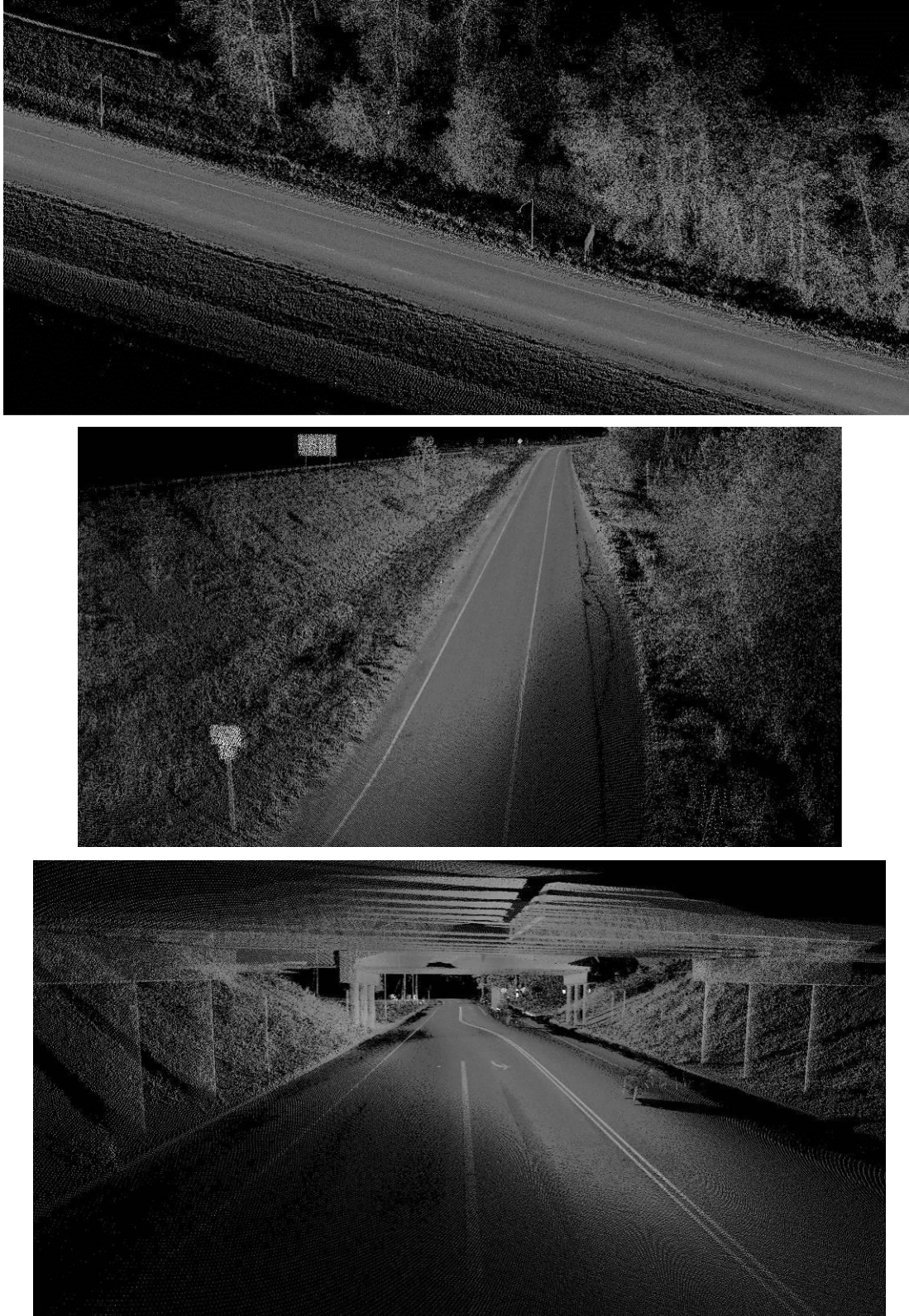
Figure A.16: Point-cloud produced by Optech Lynx mobile LiDAR system
