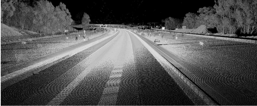
Figure 1.2: Example point-cloud of a highway produced by a mobile LiDAR system (Data courtesy of Terrametrix)
