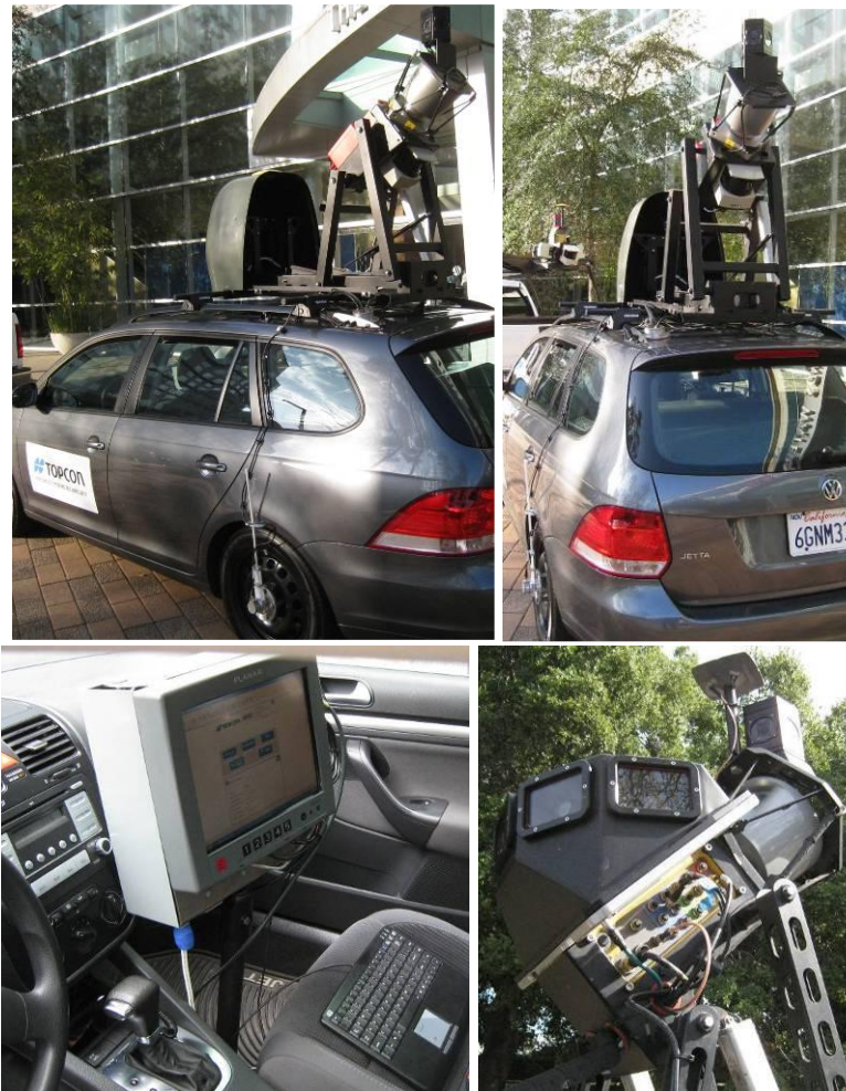
Figure A.22 Topcon IP-S2 system configured with Velodyne HDL-64E
