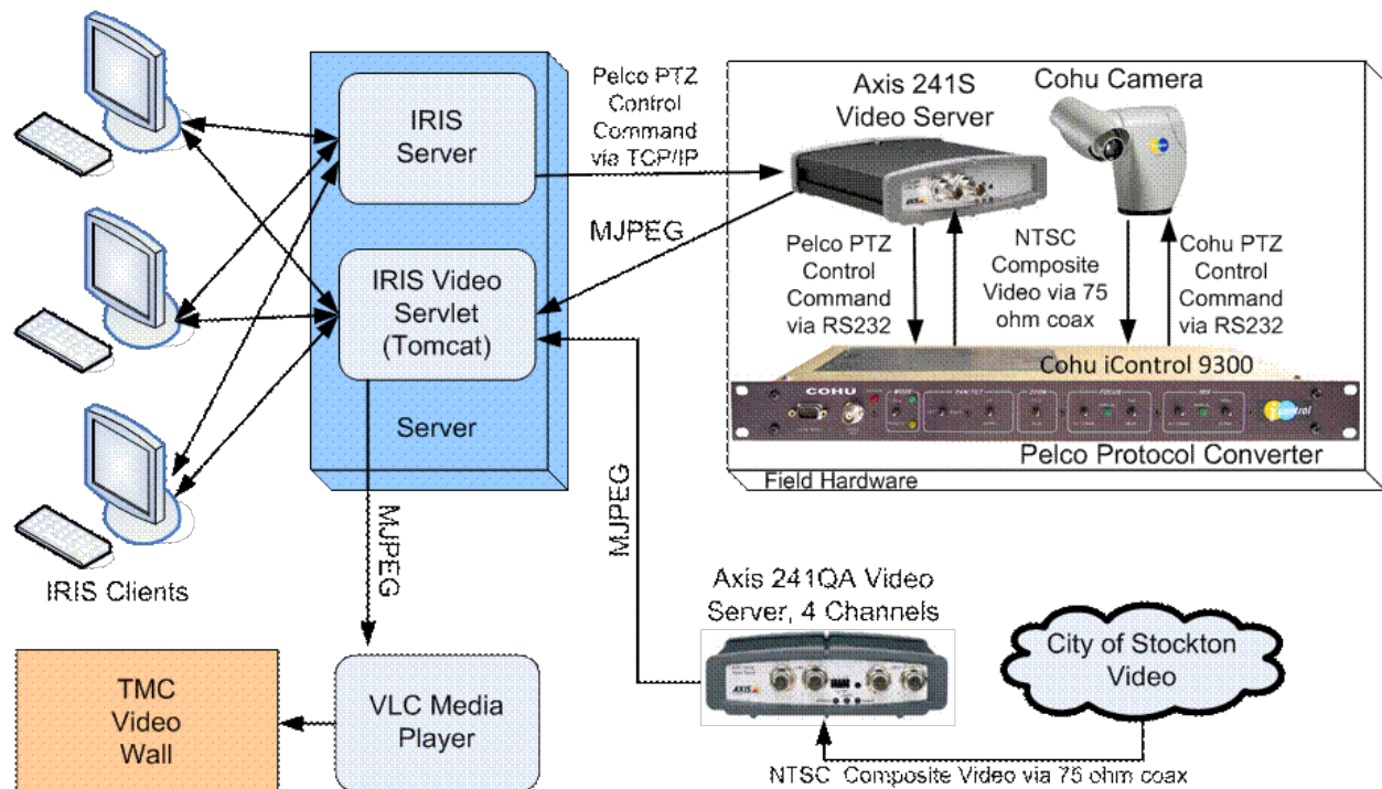
Figure 3.18: D10 video architecture
