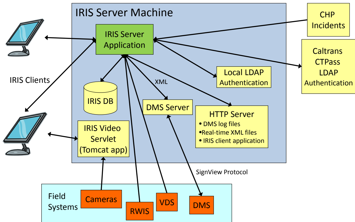
Figure 3.12: Data flow among IRIS applications
