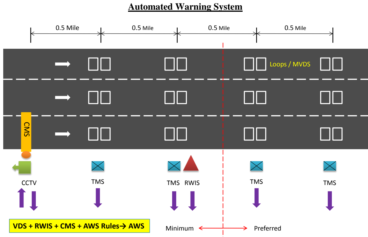
Figure 3.6: Typical Automated Warning System (AWS) configuration
