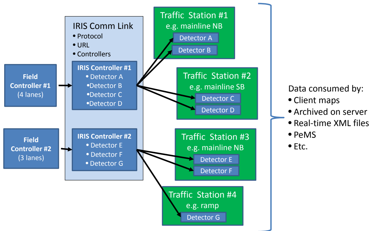
Figure 3.9: VDS configuration
