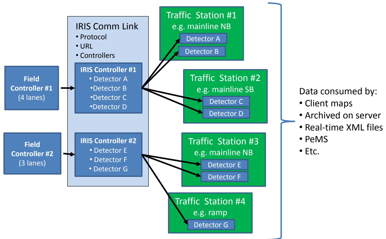
Figure 3.9: VDS configuration
