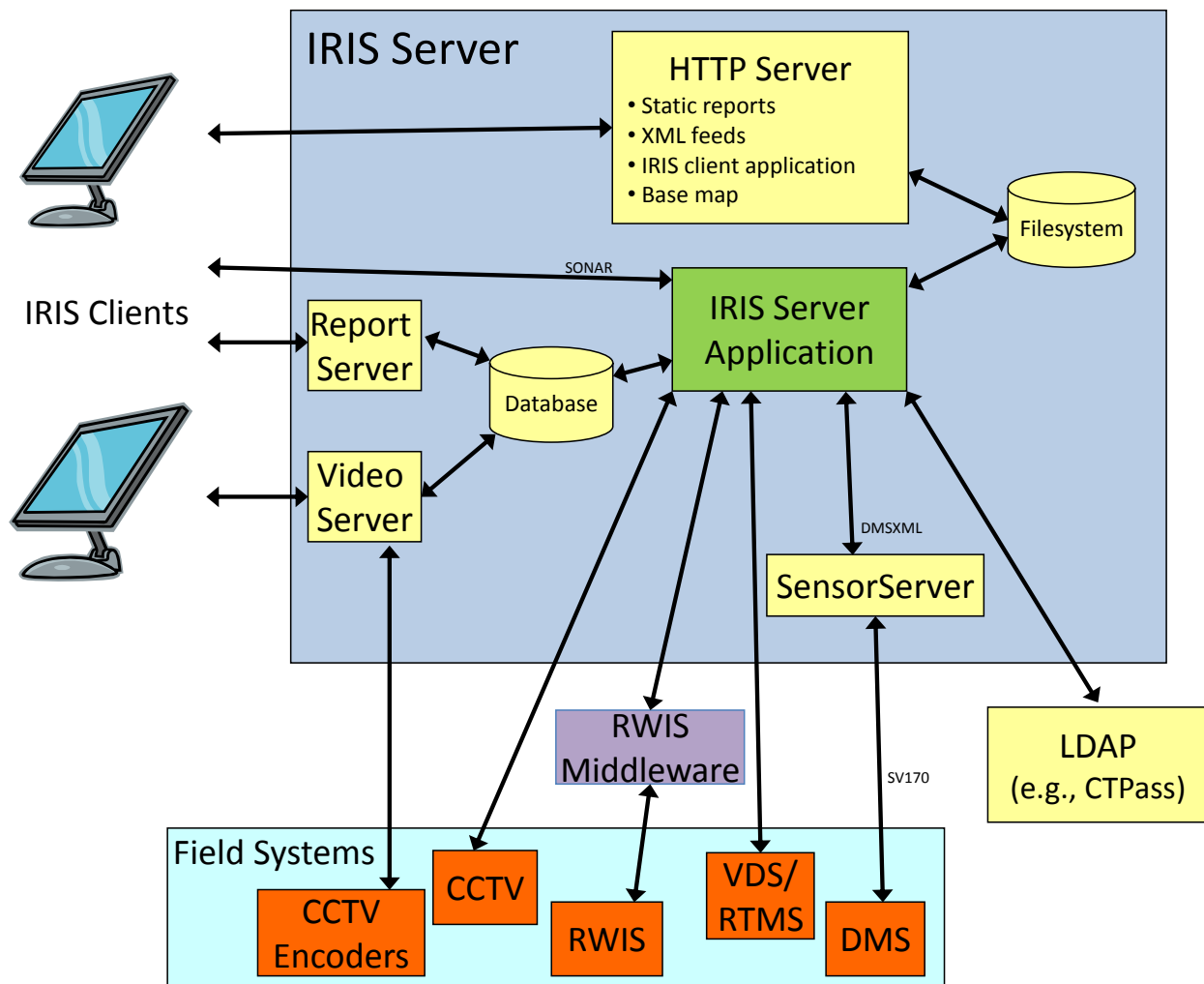
Figure 3.12: General data flow in an IRIS deployment
