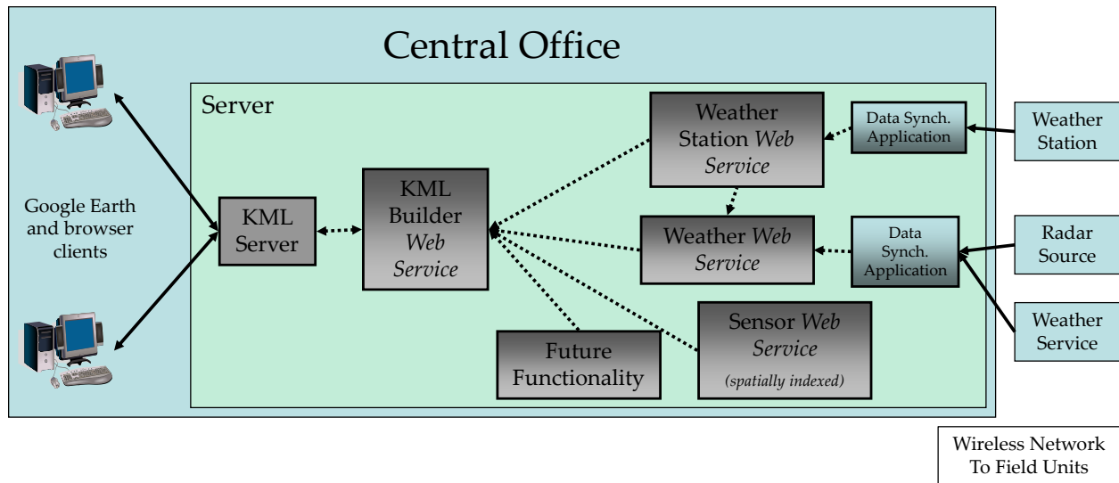
Figure 2.1: Central office architecture
