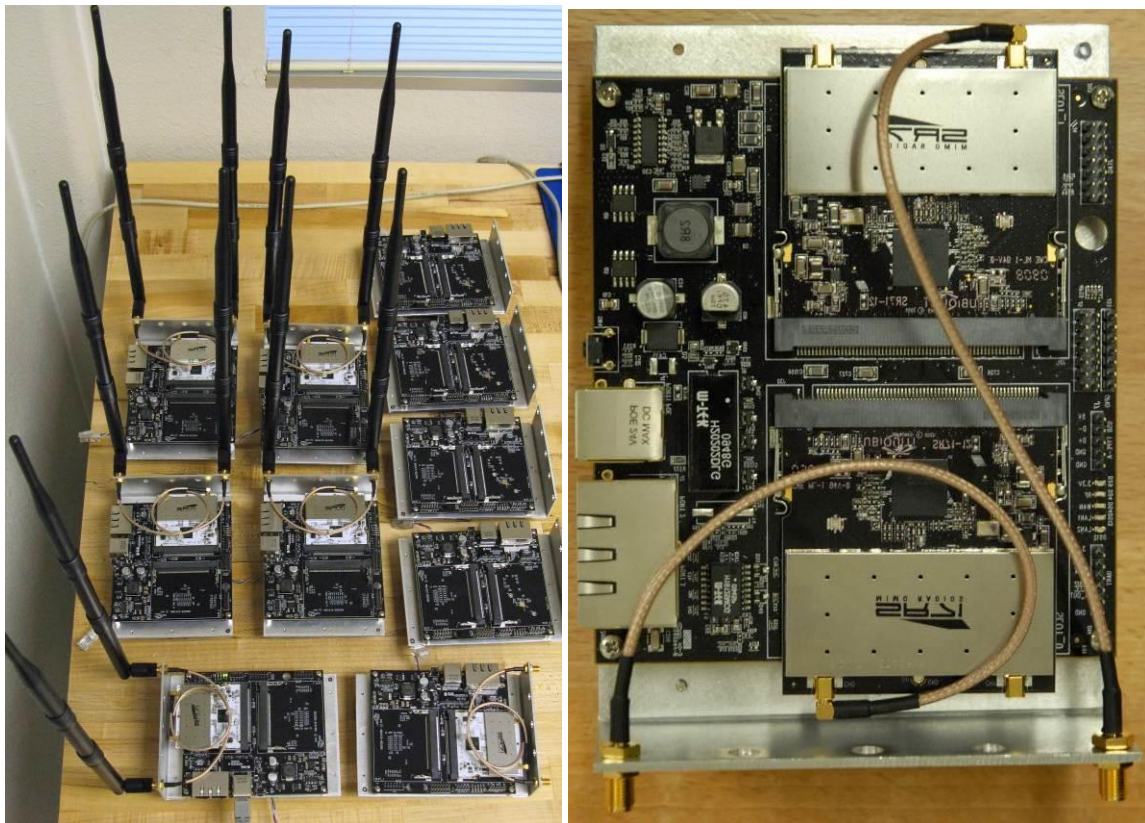
Figure 3.7: AHMCT 5.8 GHz mesh network experiment setup
