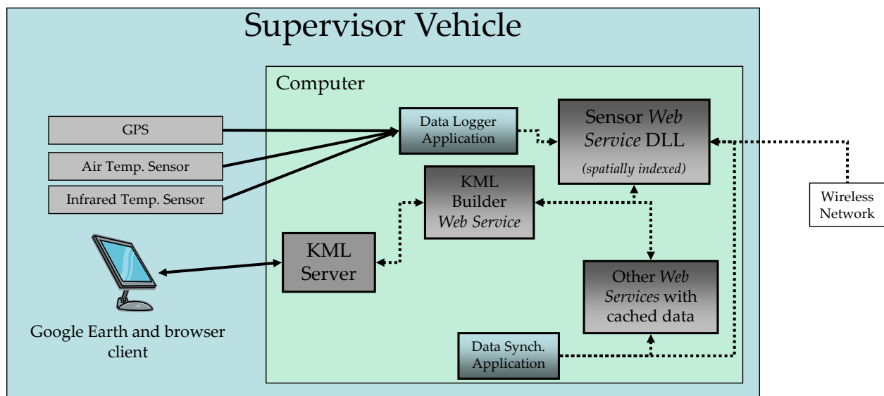
Figure 2.2: Supervisor vehicle architecture
