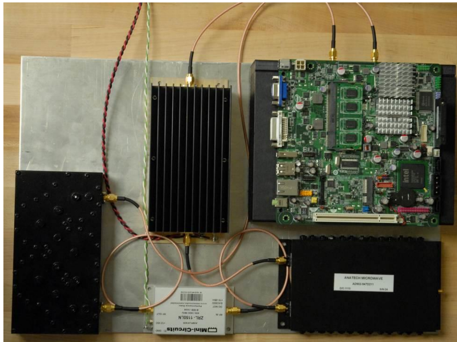
Figure 3.1: OpenBTS base station hardware implementation at AHMCT
