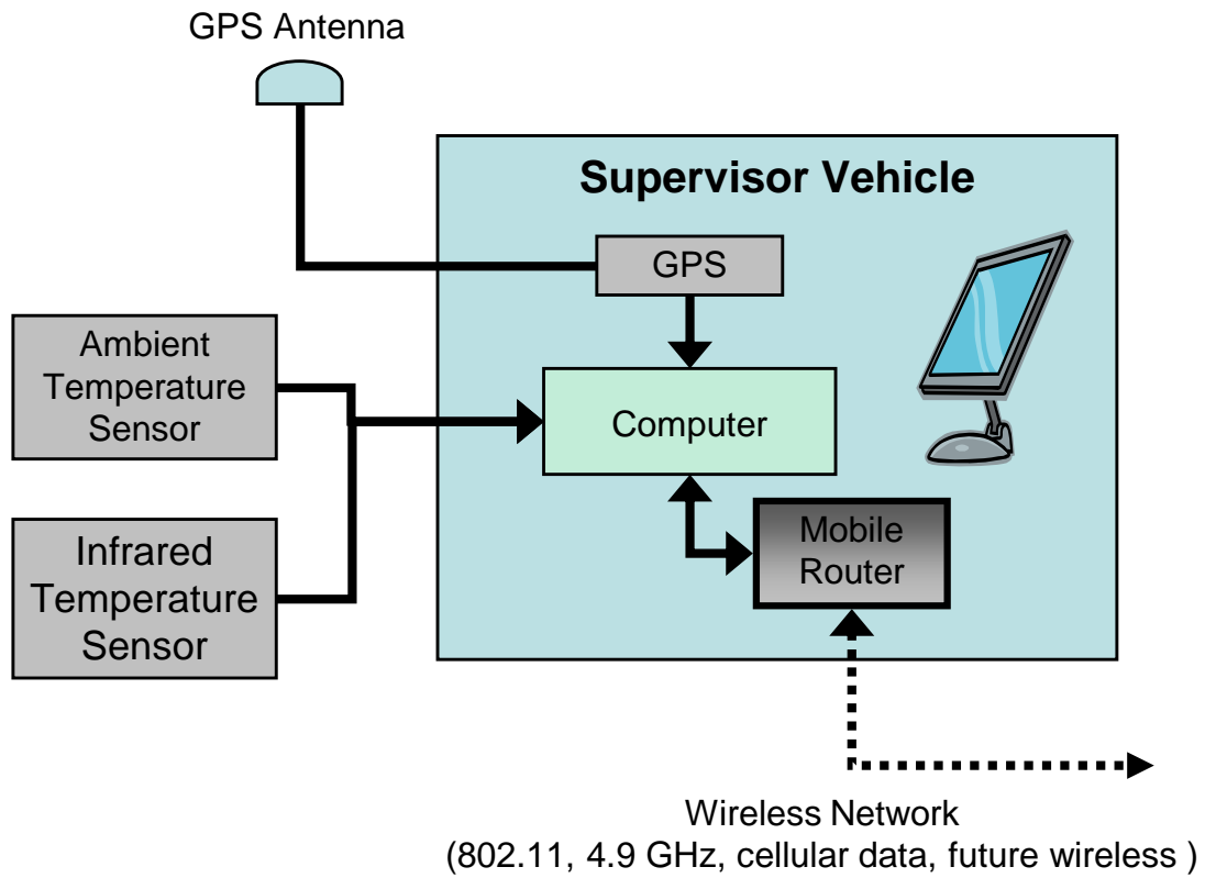
Figure 2.5: Supervisor vehicle hardware architecture
