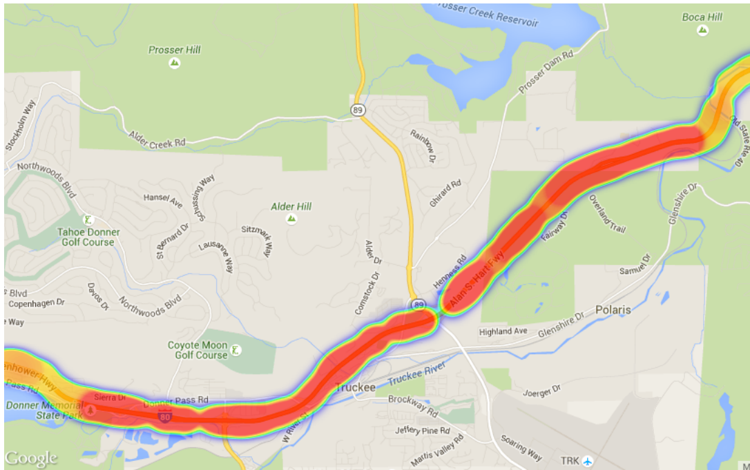
Figure D.20: Verizon signal strength for Interstate 80, Donner Lake to Old SR 40 (survey: June 21, 2013 from 10:30 – 11:45)
