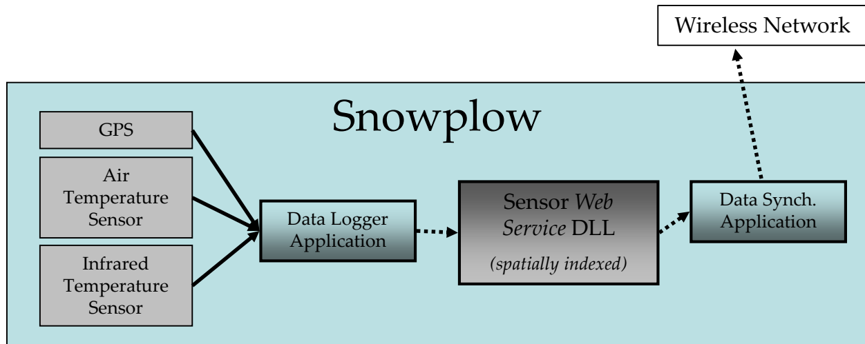
Figure 2.3: Snowplow vehicle reduced architecture
