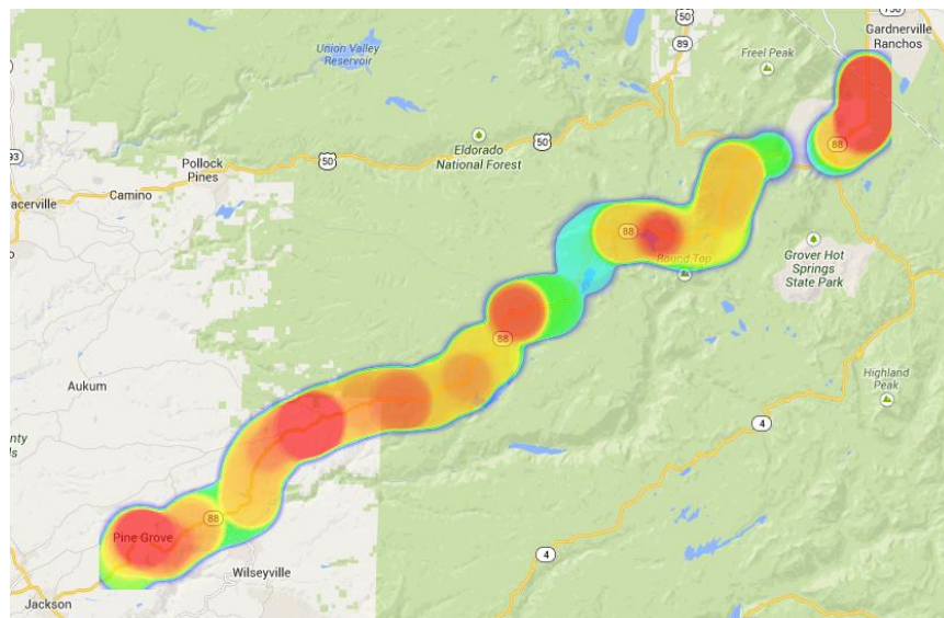
Figure D.23: AT&T signal strength for State Route 88 near Caples Lake maintenance yard (survey: August 3, 2013 from 12:25 – 13:52)
