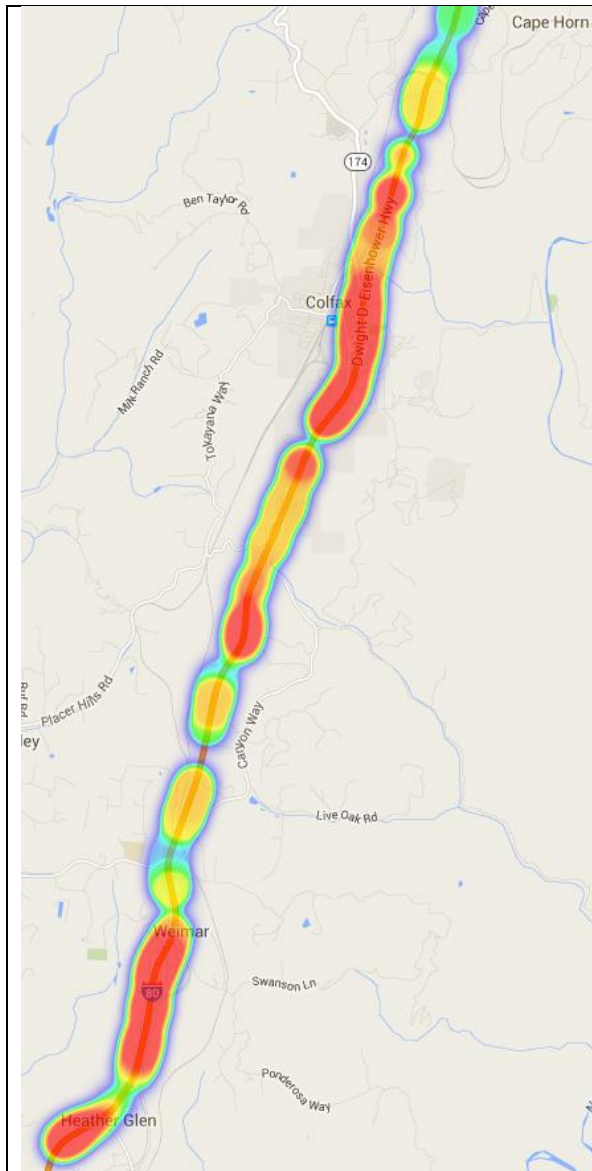
Figure D.7: AT&T signal strength for Interstate 80, Heather Glen to Cape Horn (survey: June 21, 2013 from 10:30 – 11:45)
