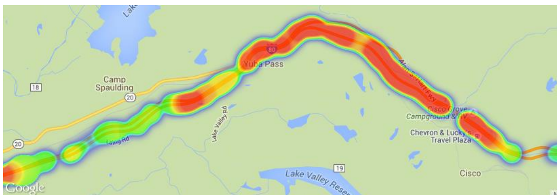
Figure D.13: AT&T signal strength for Interstate 80, Emigrant Gap to Cisco (survey: June 21, 2013 from 10:30 – 11:45)
