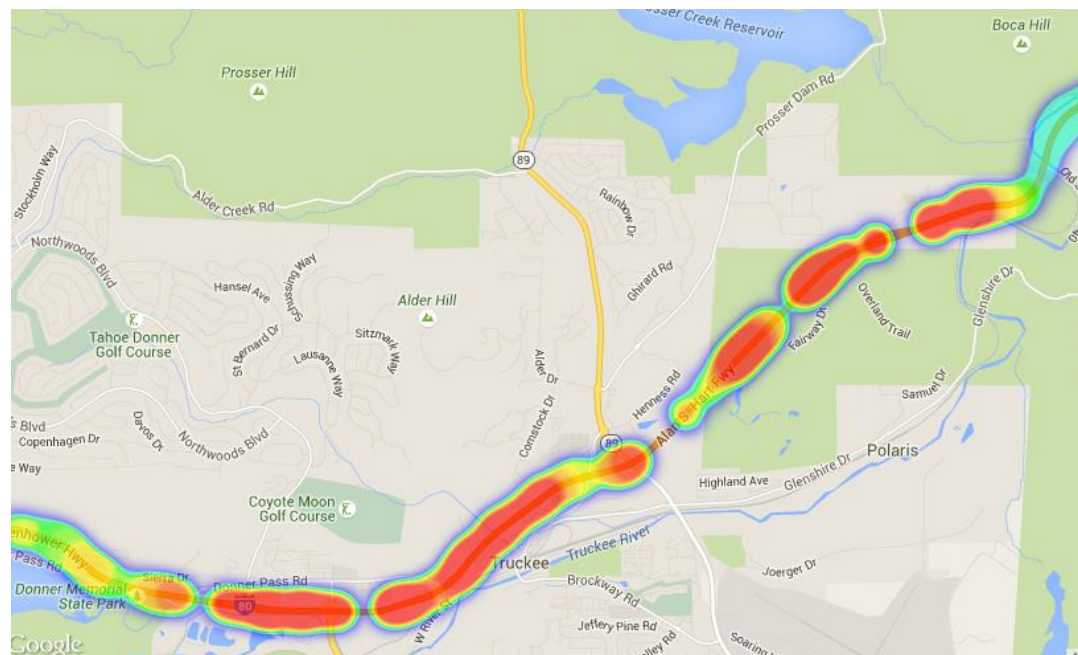
Figure D.19: AT&T signal strength for Interstate 80, Donner Lake to Old SR 40 (survey: June 21, 2013 from 10:30 – 11:45)
