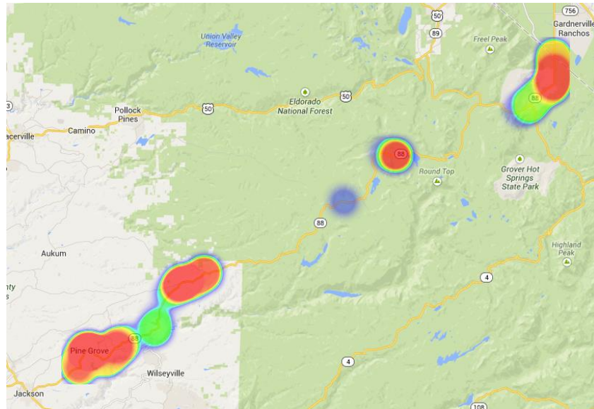
Figure D.23: AT&T signal strength for State Route 88 near Caples Lake maintenance yard (survey: August 3, 2013 from 12:25 – 13:52)
