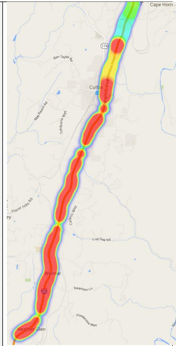
Figure D.8: Verizon signal strength for Interstate 80, Heather Glen to Cape Horn (survey: June 21, 2013 from 10:30 – 11:45)
