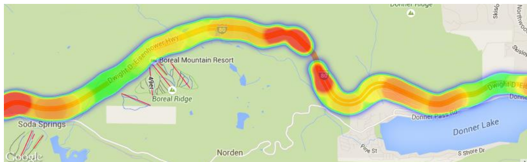
Figure D.18: Verizon signal strength for Interstate 80, Kingvale to Donner Lake (survey: June 21, 2013 from 10:30 – 11:45)
