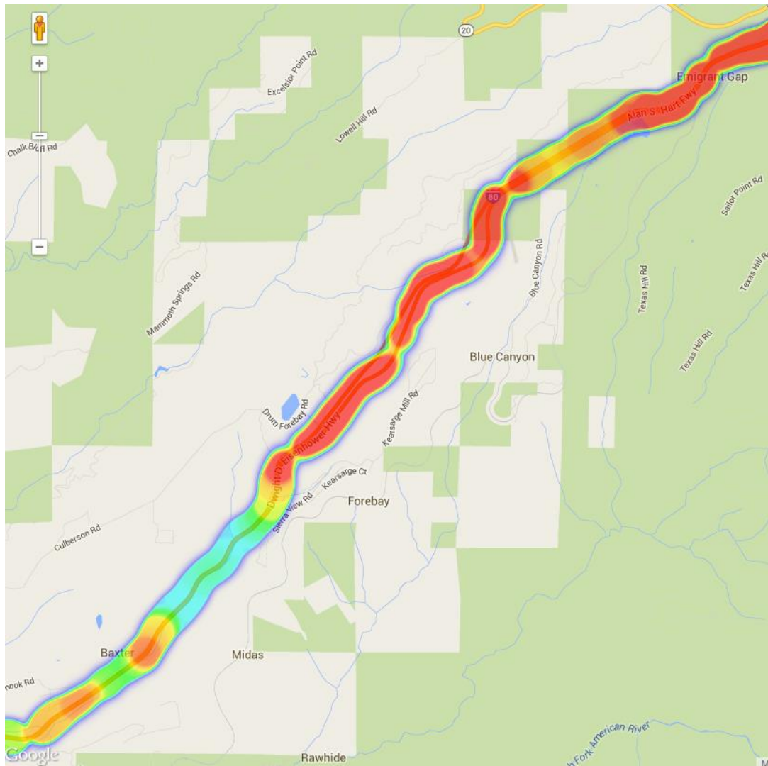
Figure D.12: Verizon signal strength for Interstate 80, Alta to Emigrant Gap (survey: June 21, 2013 from 10:30 – 11:45)
