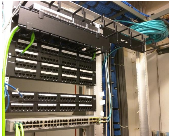
Figure 2.2: Networking equipment in 13 th floor network closet
