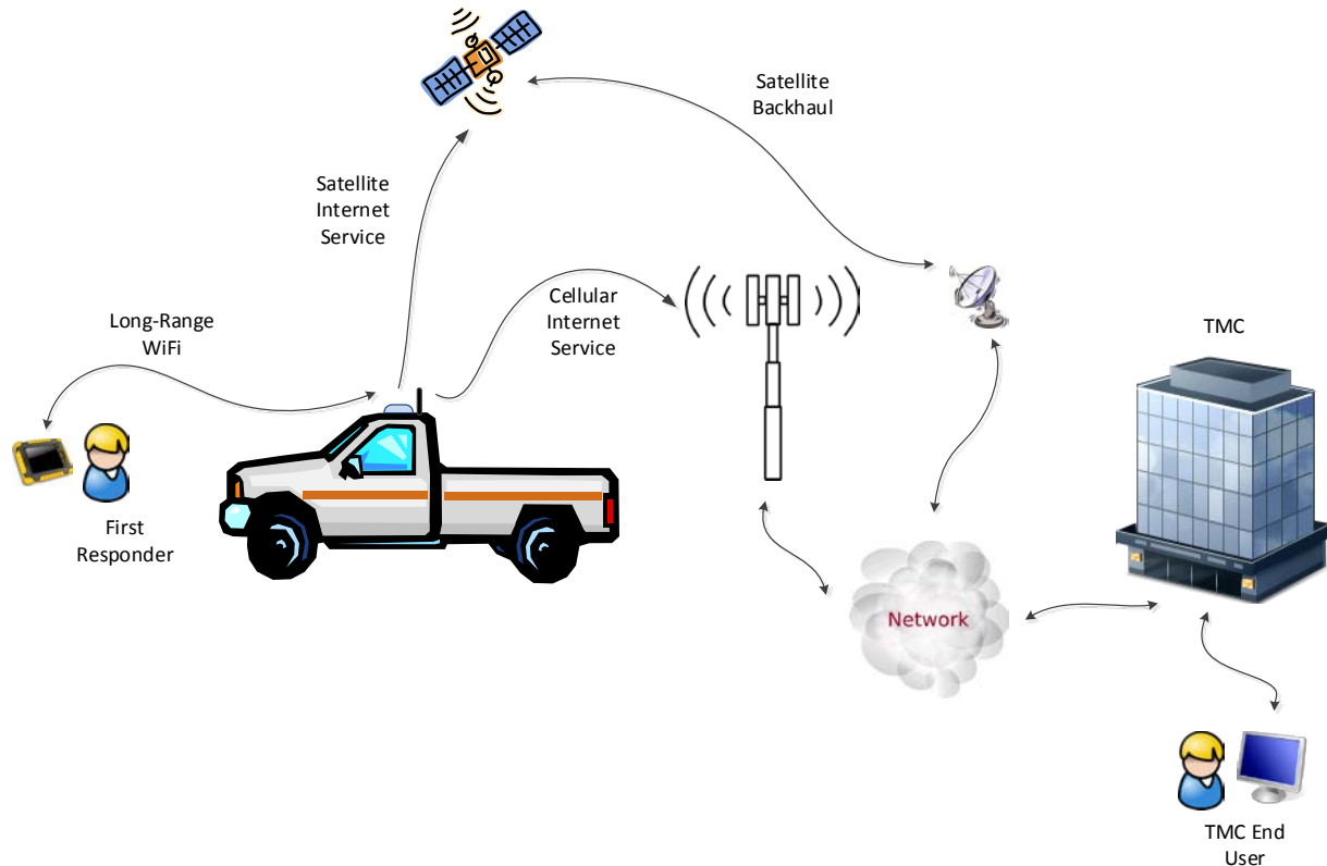
Figure 2.1: Responder concept
