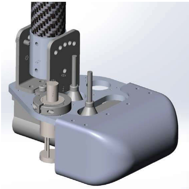
Figure 3.5: PicoMBES 120 sensor assembly with protective cover CAD model
