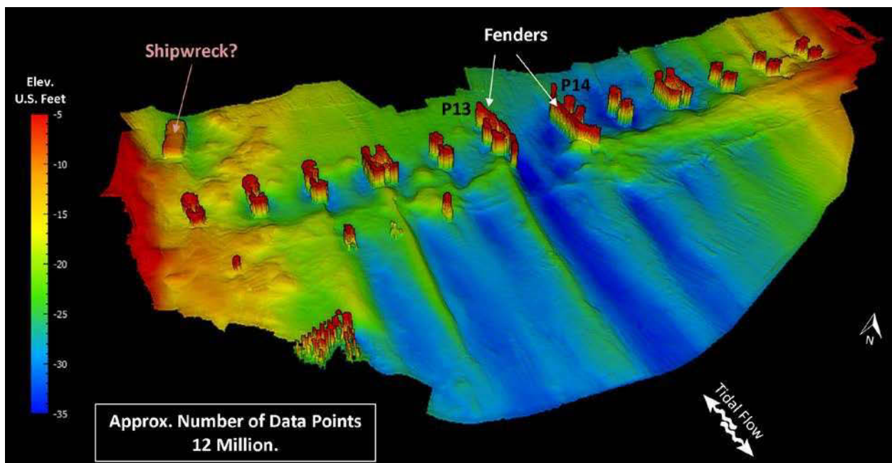
Figure 3.23: 3D view of bathymetric contour plot elevation Napa River Bridge SR37
