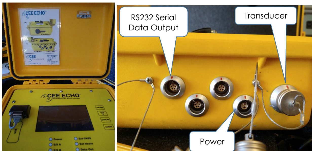
Figure 3.17: CEE Echo computer. Right image shows the RS232 serial port connection location.
