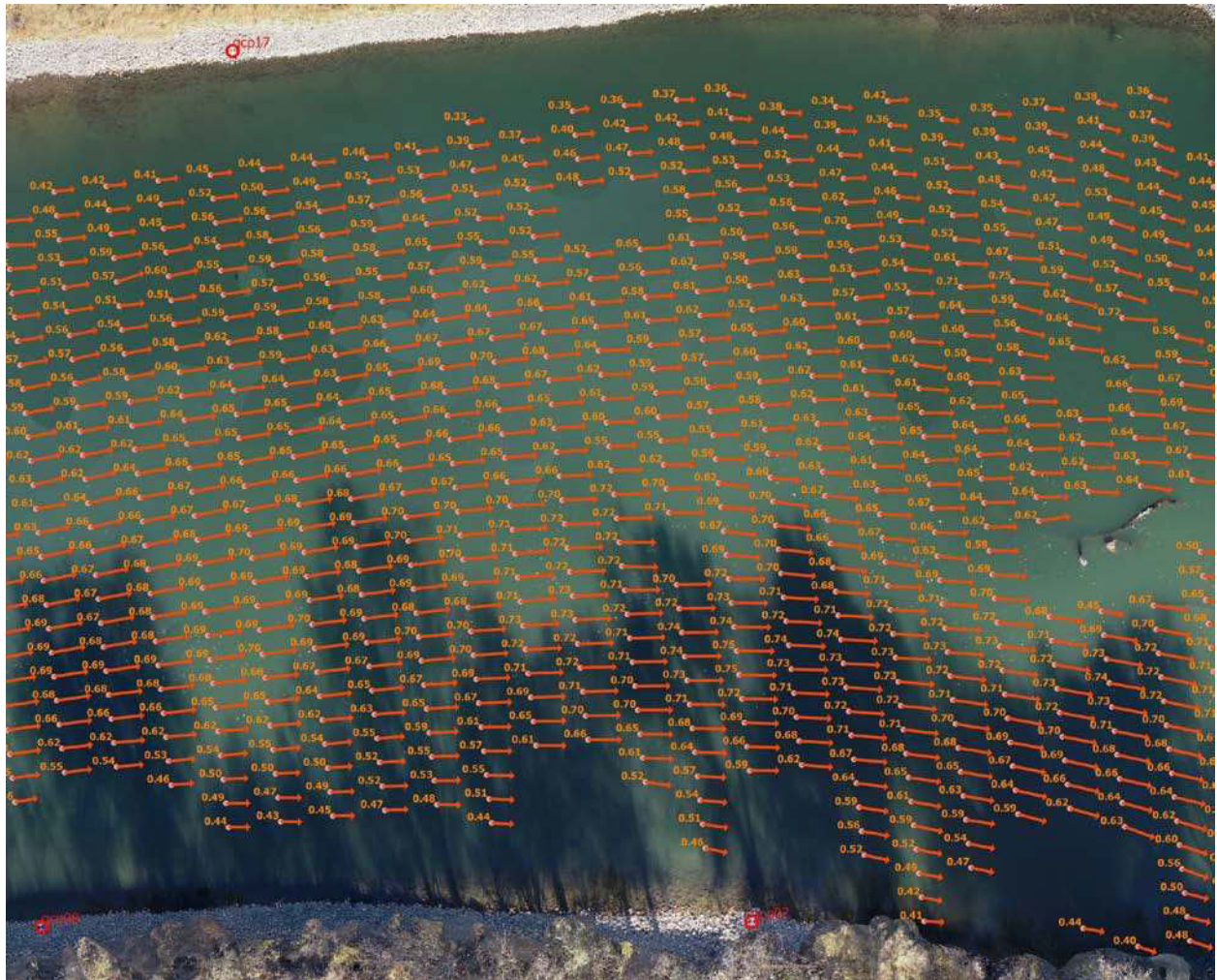
Figure 4.12: RIVER LSPIV result from a 4K video overlaid on georeferenced orthophoto in QGIS
