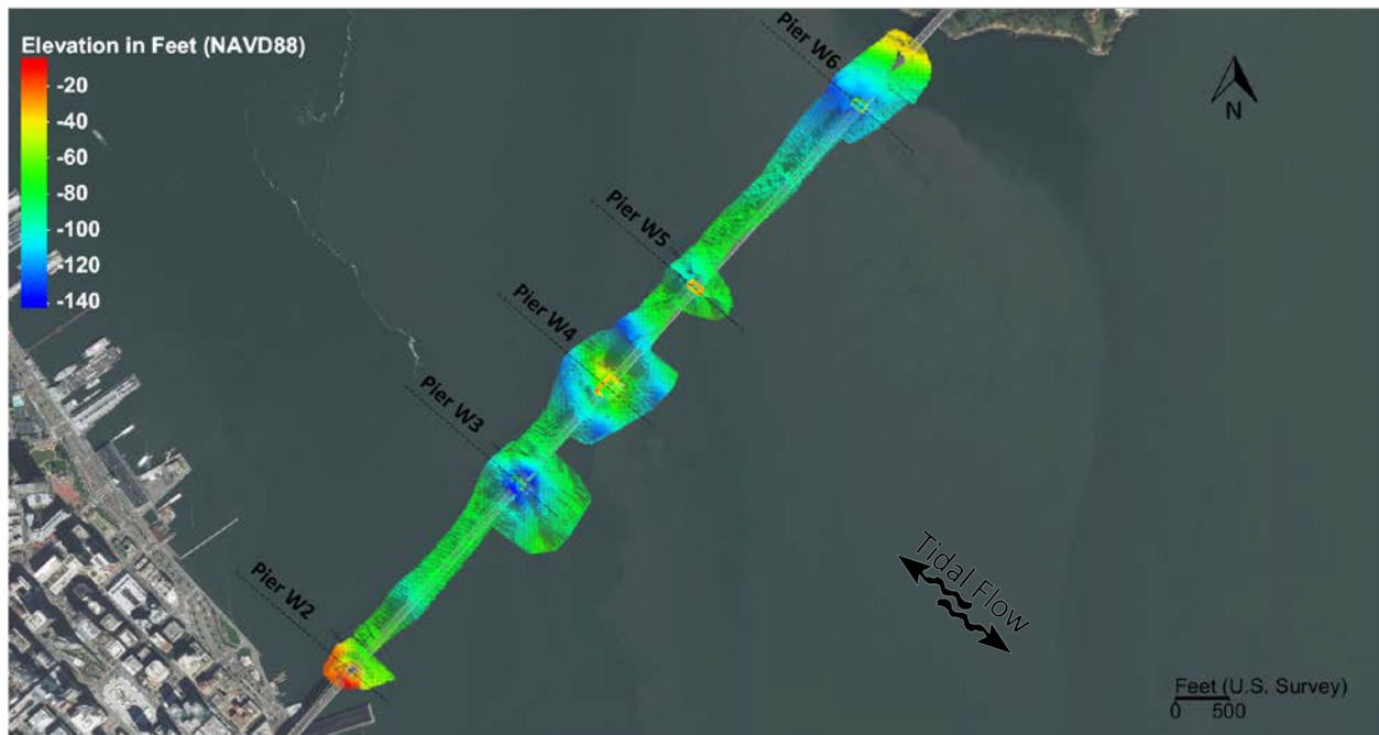
Figure 3.24: Bathymetric survey result of San Francisco-Oakland Bay Bridge, CA
