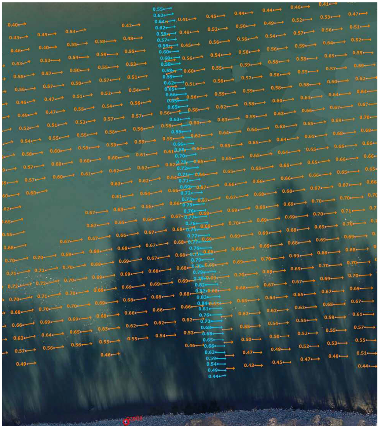
Figure 4.15: RIVER LSPIV and ADCP result overlaid on the orthophoto. The average ADCP data are represented by light blue arrows, and the orange arrows represent LSPIV results from the 4K UAS color video. The blue text represent the surface flow estimate calculated from the average ADCP measurement values, and the orange text represents the LSPIV estimates.
