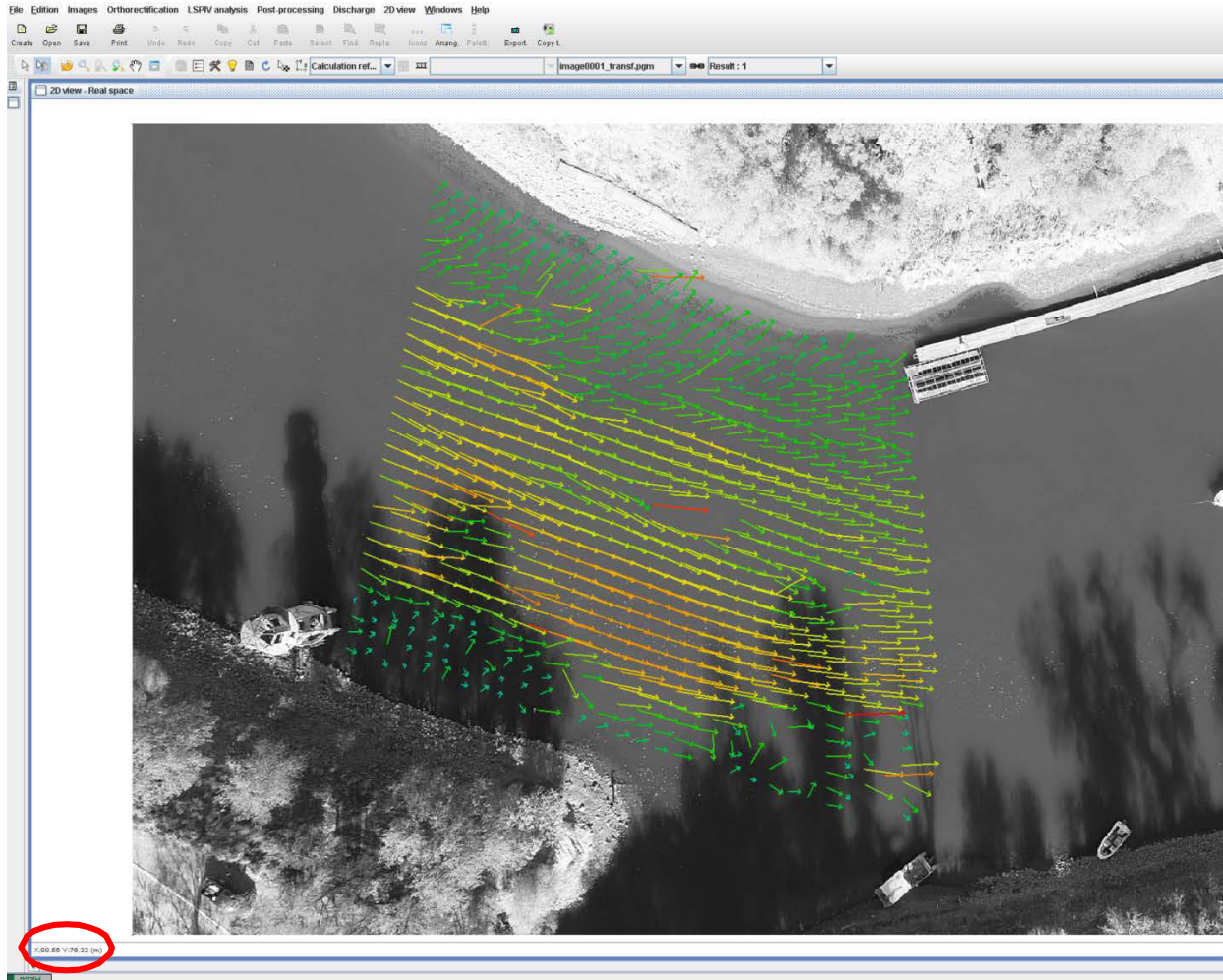
Figure 4.10: Fudaa-LSPIV GUI. The local XY coordinate values under the mouse cursor are displayed in the lower-left corner (highlighted by a red circle at the lower left corner)
