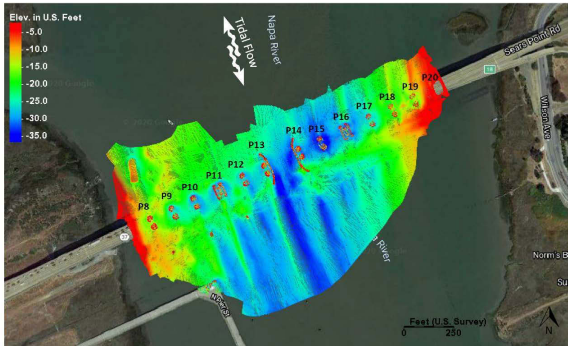
Figure 3.22: Example bathymetric survey result presented by SM&I in Caltrans ABME meeting
