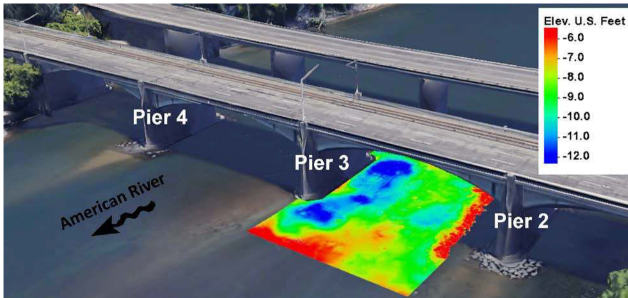
Figure 3.25: Underwater excavation before RSP installation at American River SR160 westbound
