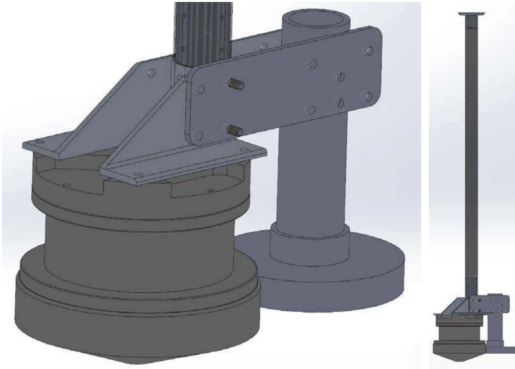
Figure 3.6: ADCP and echo sounder sensor assembly CAD model
