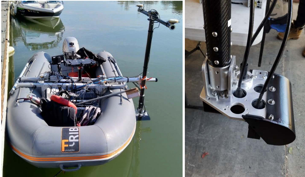
Figure 3.11: SM&I foldable boat with PicoMBES 120 sensor in water (bathymetric survey configuration). The data collection rugged laptop was removed.
