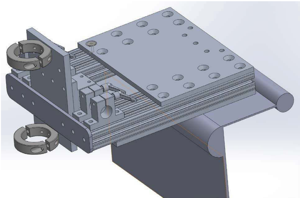
Figure 3.13: Sensor mount CAD model
