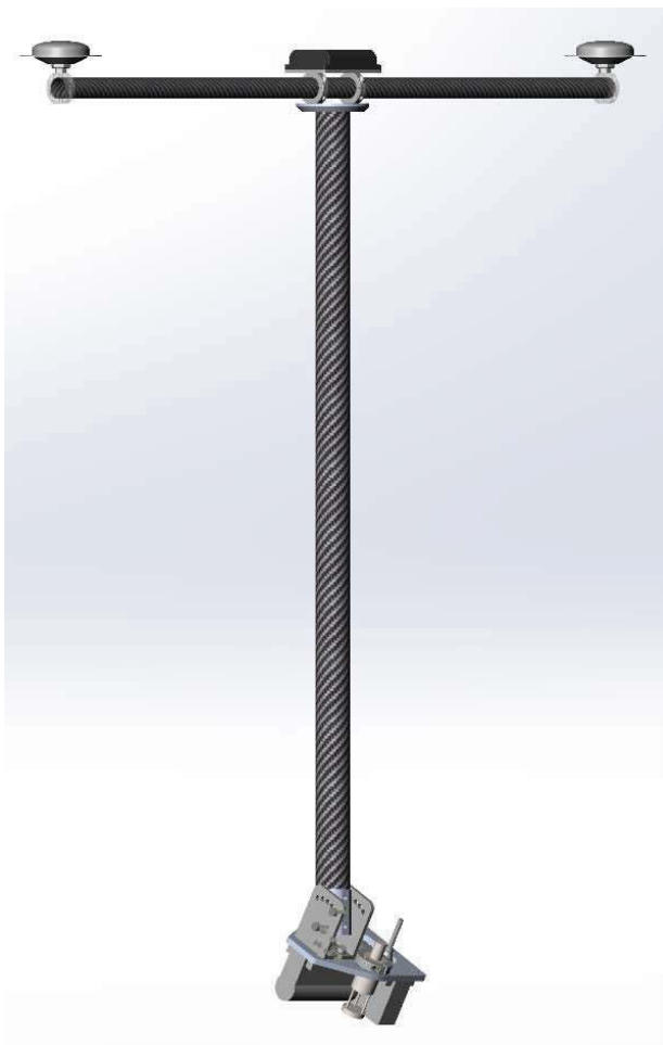
Figure 3.2: Antenna bar and PicoMBES 120 sensor assembly CAD model. The CAD model shows a 30-degree tilt of the PicoMBES 120 sensor assembly.
