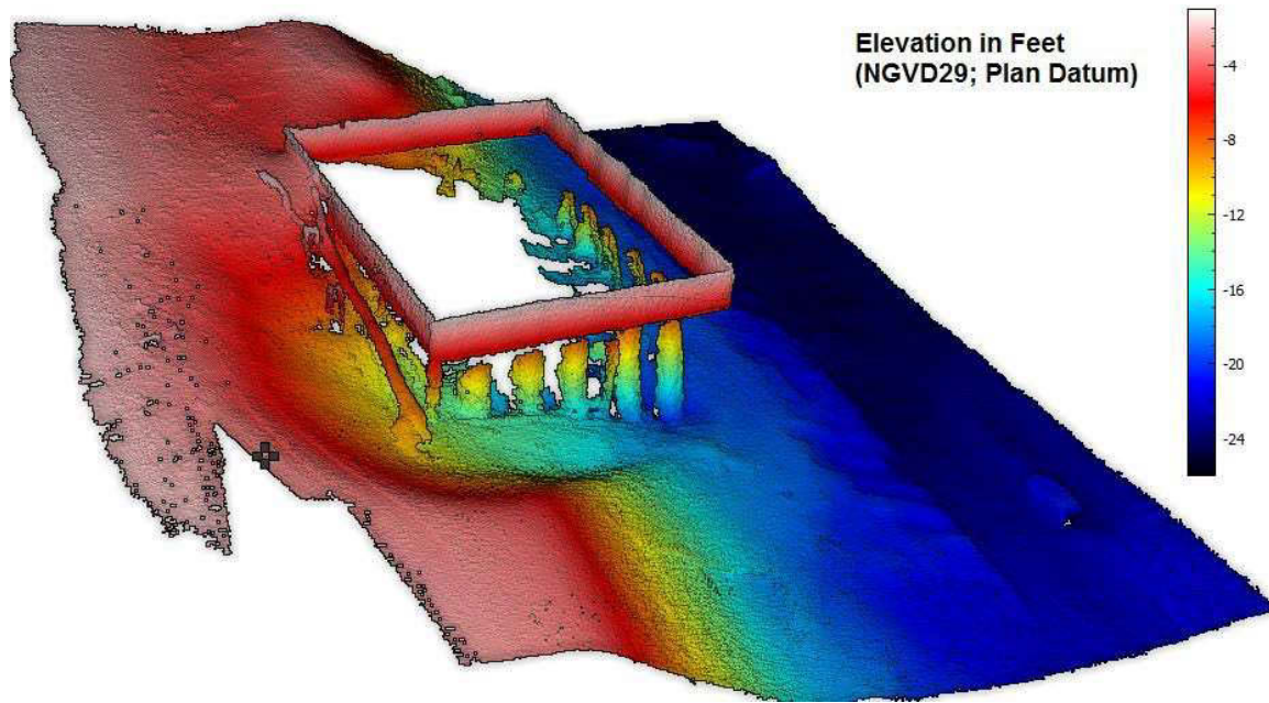
Figure 3.20: PicoMBES 120 survey of Napa River Bridge pier data using BeamworX software
