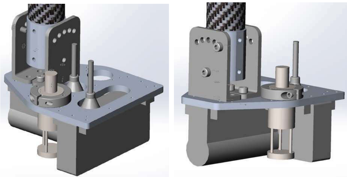
Figure 3.3: PicoMBES 120 sensor assembly CAD model
