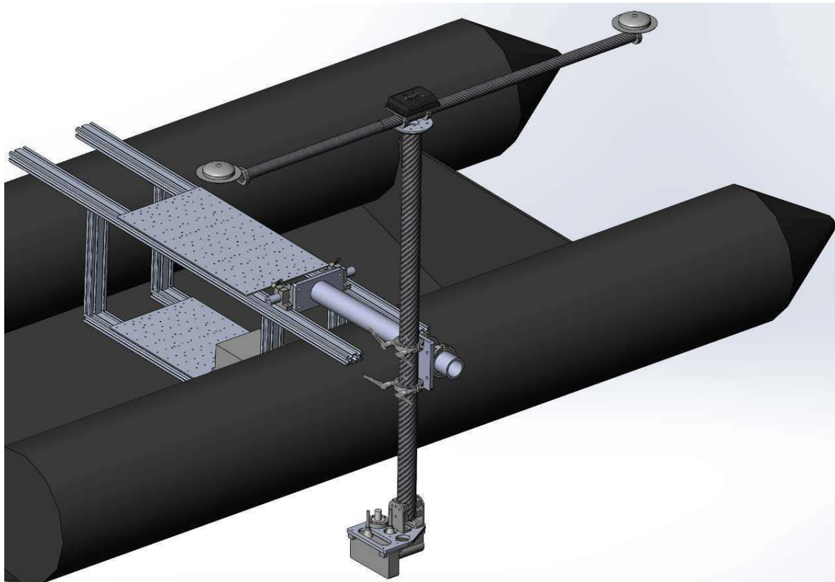
Figure 3.8: CAD model of component mounting platform in a foldable boat
