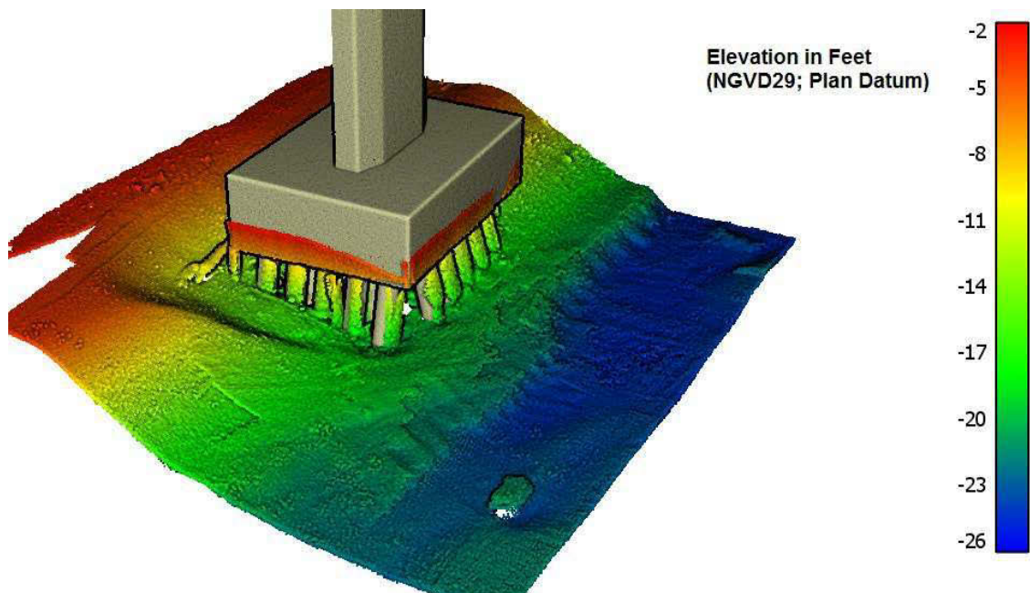
Figure 3.21: PicoMBES 120 survey of Napa River Bridge pier data overlaid on CAD model
