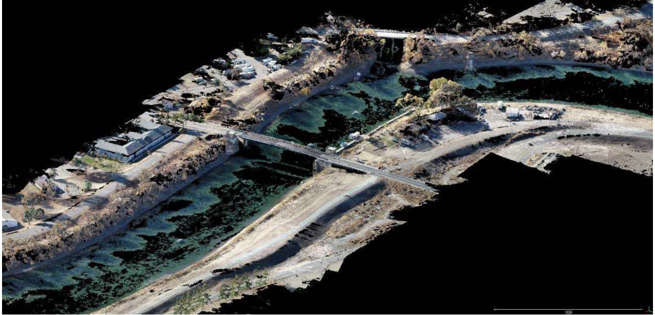
Figure 4.6: SR113 pilot study site point cloud (64 million points) created by WebODM software using 679 aerial images
