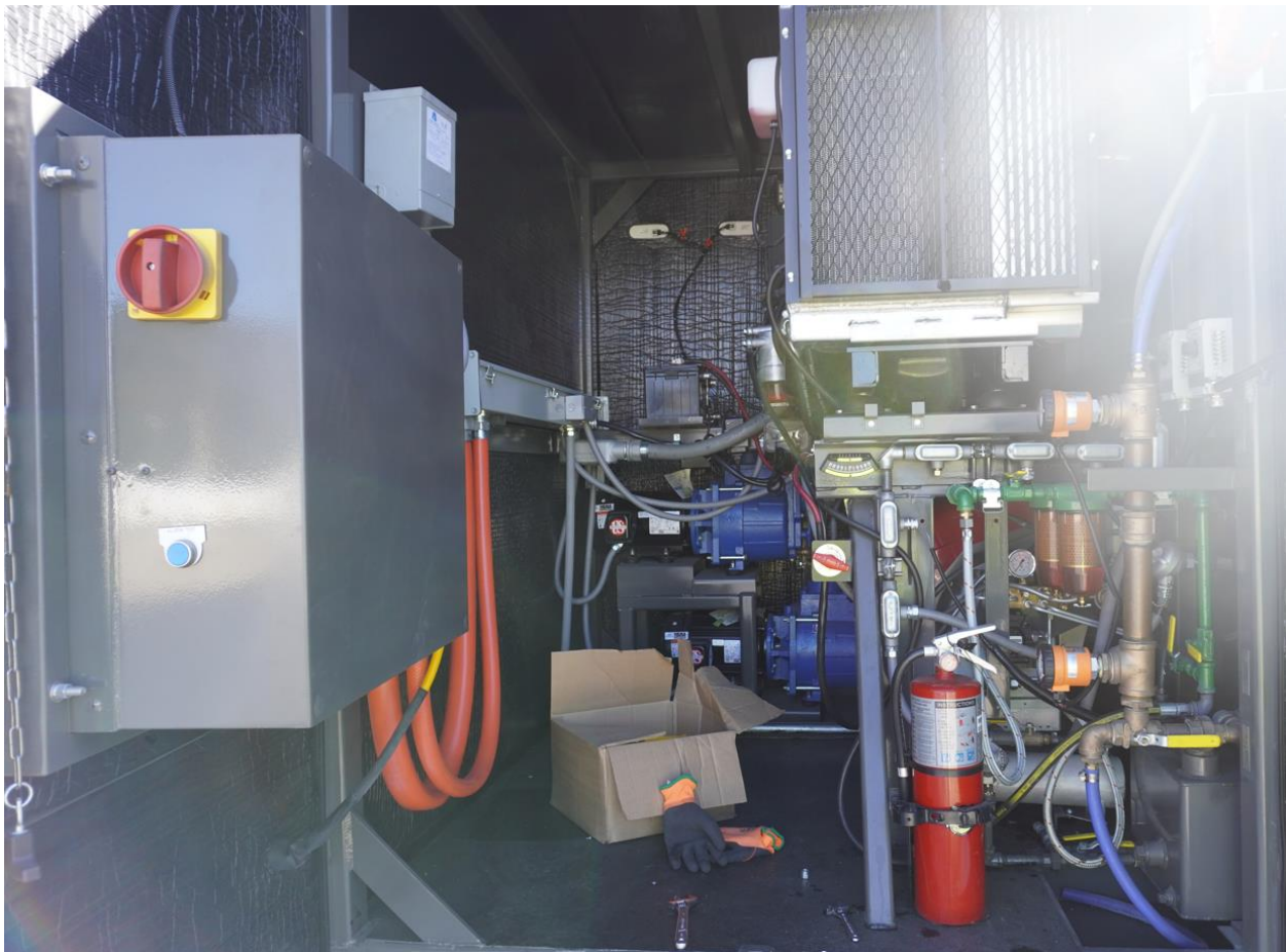
Figure 3.3: SND900 operating enclosure
