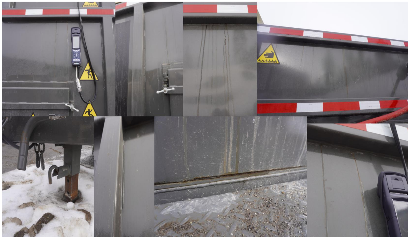
Figure 4.2: Examples of rust and small water leaks on the Snow Dragon
