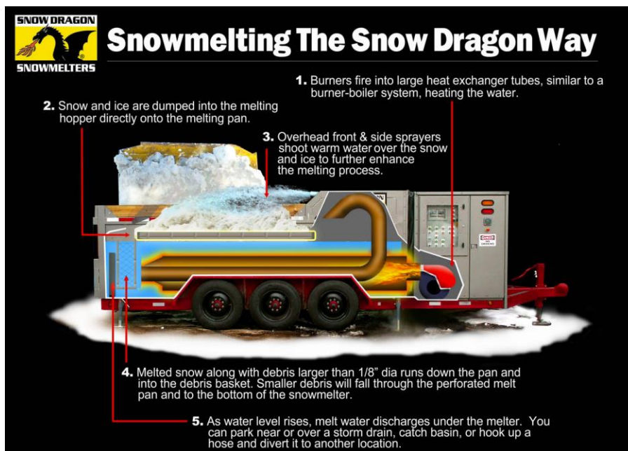
Figure 2.3: How the Snow Dragon works. Image courtesy of the Snow Dragon manufacturer.
