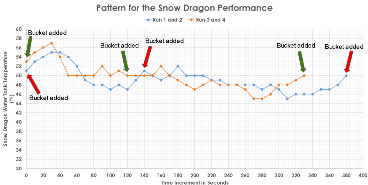
Figure 5.4: Snow Dragon performance pattern. Red arrow indicates data line “Run 1 and 2”. Green arrow indicates data line “Run 3 and 4”. “Bucket added” means a bucket was being dumped into the Snow Dragon. All test runs were for snow with less sand.
