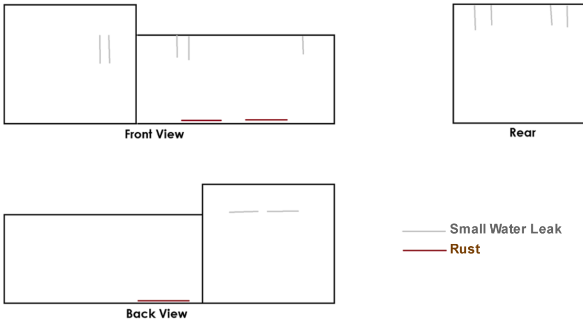
Figure 4.3: Locations where rust and small water leaks were detected on the Snow Dragon. Note that these spots only reflect problems documented on February 2.
